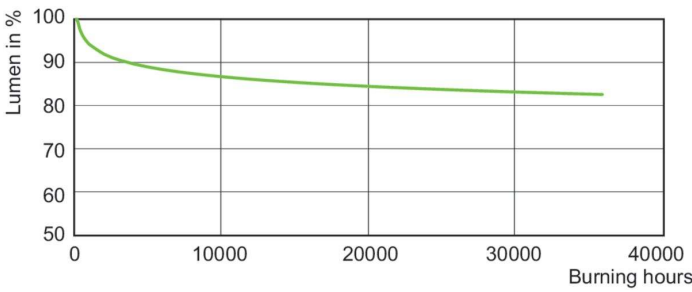
Lumen Maintenance Diagram - Allstart Energy Adv 330W ED37 CL 1SL
