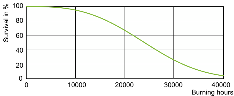
Life Expectancy Diagram - MHC150/C/U/MP/3K ALTO 12PK
