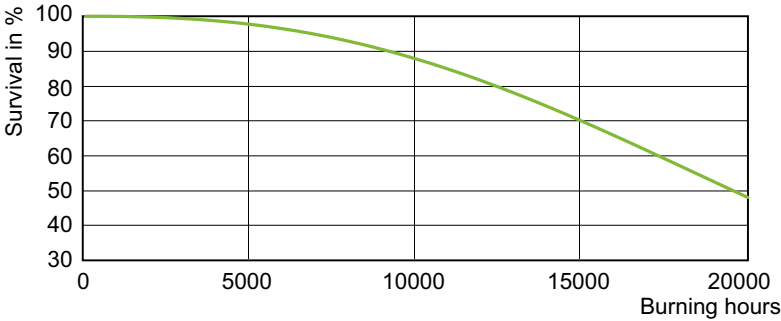
Life Expectancy Diagram - MHC100/C/U/MP/3K ELITE
