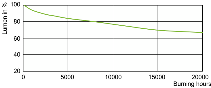
Lumen Maintenance Diagram - CDM 315/U/O/4K ED37 6PK
