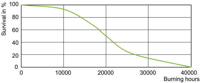
Life Expectancy Diagram - CDM 315/U/O/4K ED37 6PK
