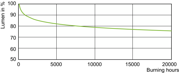
Lumen Maintenance Diagram - CDM70/U/PS/4K ED23.5 - Elite
