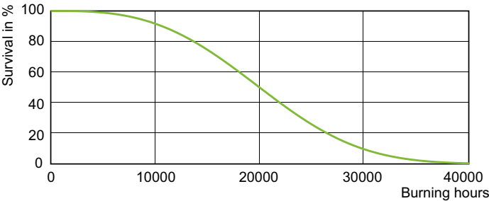
Life Expectancy Diagram - CDM70/U/PS/4K ED23.5 - Elite
