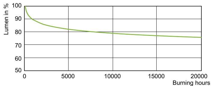
Lumen Maintenance Diagram - CDM100/U/PS/4K ED23.5 - Elite
