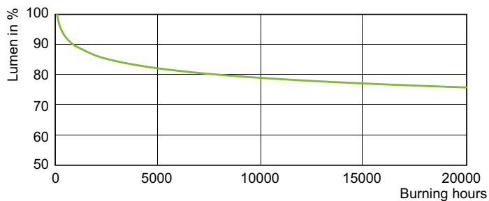
Lumen Maintenance Diagram - MHC100/U/HR/4K ED28 - Elite
