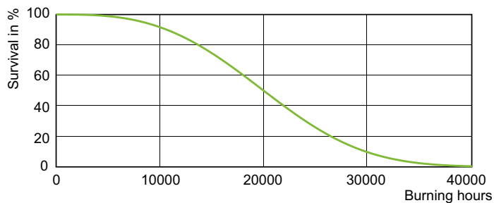
Life Expectancy Diagram - MHC100/U/HR/4K ED28 - Elite
