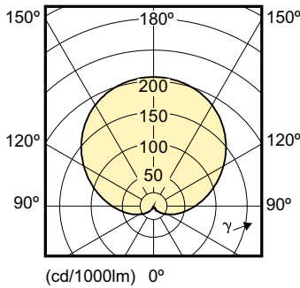
Light Distribution Diagram - CorePro LEDbulb 9-60W E27 827
