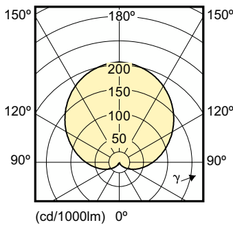
Light Distribution Diagram - LEDBulb 9.5-60W E27 3000K 220-240V A55
