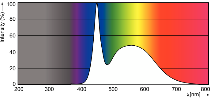
Spectral Power Distribution Colour - LEDBulb 12.5-75W E27 6500K 220-240V A67
