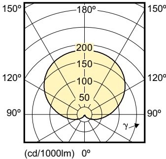
Light Distribution Diagram - LEDBulb 12.5-75W E27 6500K 220-240V A67
