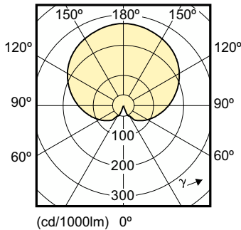
Light Distribution Diagram - CorePro luster ND 6-40W E14 827 P48 FR
