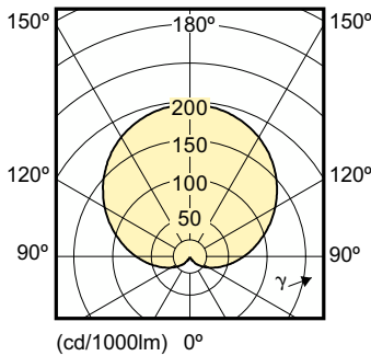
Light Distribution Diagram - CorePro LEDbulb 6-40W E27 827
