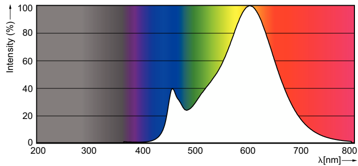
Spectral Power Distribution Colour - CorePro LEDbulb 6-40W E27 827
