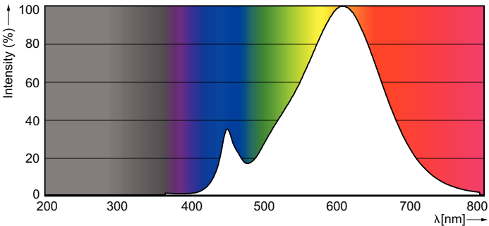
Spectral Power Distribution Colour - CorePro LEDspotMV D 4.5-40W 827 R50 36D
