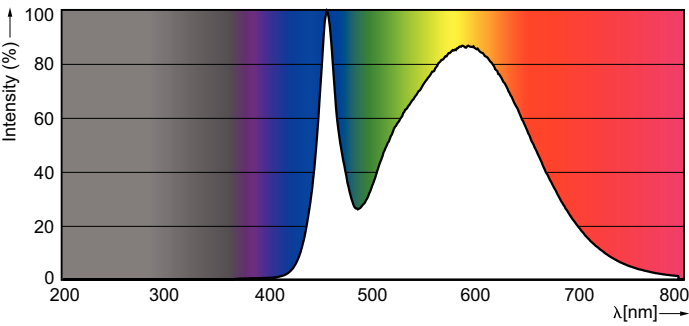
Spectral Power Distribution Colour - MAS LEDtube PERF 600mm 10.5W840 T8 C
