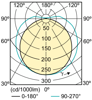
Light Distribution Diagram - MAS LEDtube PERF 600mm 10.5W840 T8 C
