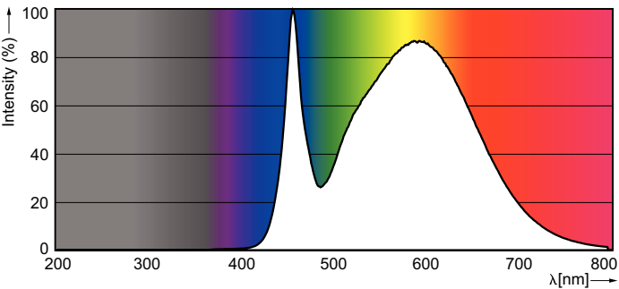
Spectral Power Distribution Colour - MAS LEDtube PERF 1200mm 21W840 T8 C
