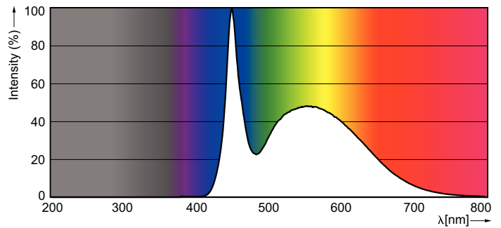
Spectral Power Distribution Colour - MAS LEDtube 1500mm SO 20W 865 T8
