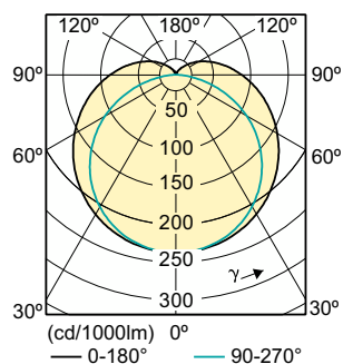
Light Distribution Diagram - ESSENTIAL LEDtube 600mm 10W865 T8 AP I
