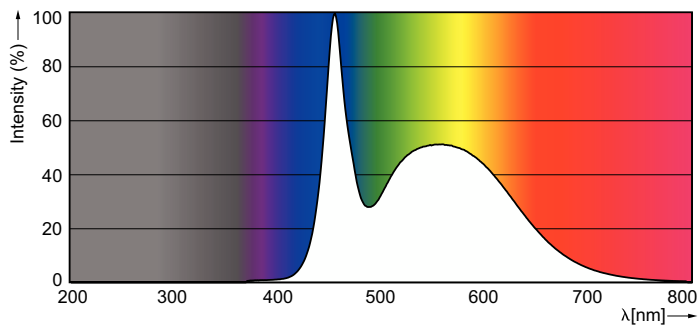
Spectral Power Distribution Colour - ESSENTIAL LEDtube 600mm 10W865 T8 AP I
