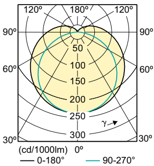
Light Distribution Diagram - ESSENTIAL LEDtube 600mm 10W865 T8 AP I
