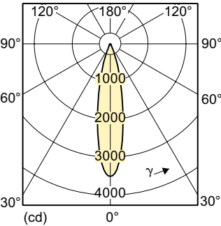
Light Distribution Diagram - 120V PAR30S 12.5W 25D 3000K 780 CW SO
