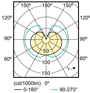
Light Distribution Diagram - SlimStyle A21 13W E26 2700K 120V ES
