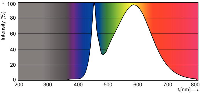
Spectral Power Distribution Colour - 120V PAR38 17W 25D 4000K 1200 D AF SO
