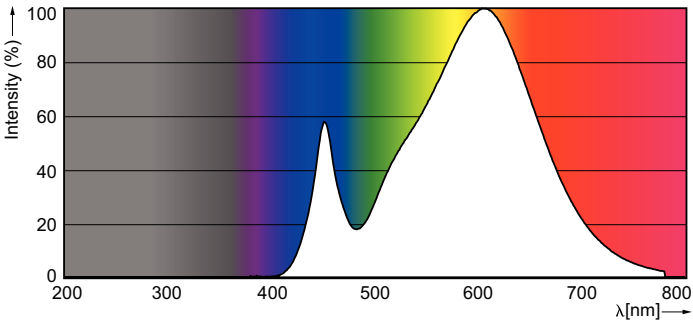
Spectral Power Distribution Colour - LED 60W E27 WW 230V R63 36D DIM SRT4
