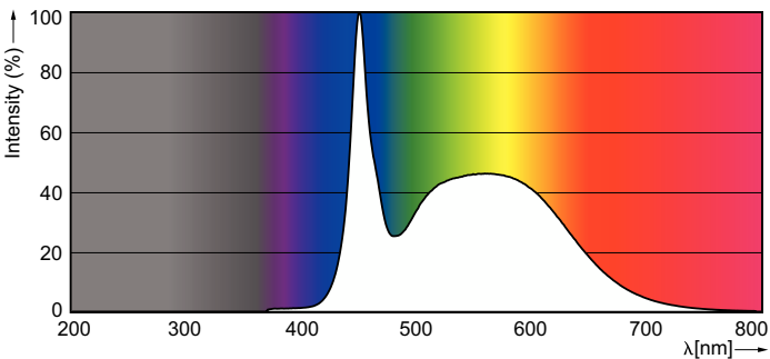
Spectral Power Distribution Colour - MAS LEDtube 1500mm HO 23W865 T8
