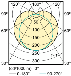
Light Distribution Diagram - 10.5T8/36-3500 IF 10/1
