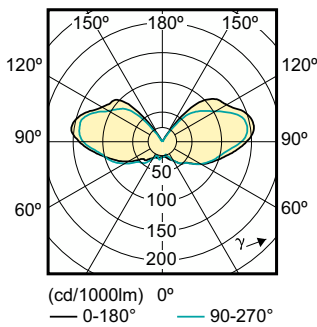
Light Distribution Diagram - LED Capsule 1.2W G4 WH AU 1PF
