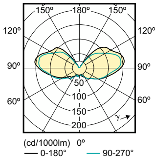
Light Distribution Diagram - LED Capsule 1.2W G4 WH AU 1PF
