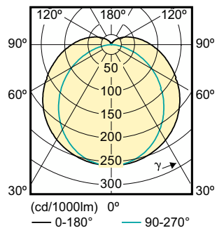
Light Distribution Diagram - MAS LEDtube 1200mm SO 14.5W 865 T8 ROT
