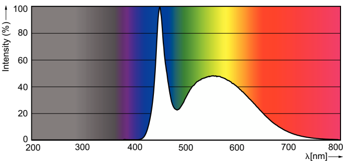
Spectral Power Distribution Colour - MAS LEDtube 1200mm SO 14.5W 865 T8 ROT
