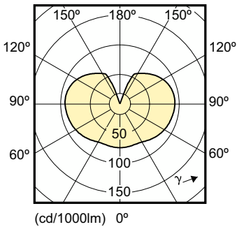
Light Distribution Diagram - 120V 3WAY A21 20W 2700K E26
