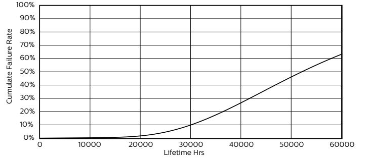
Life Expectancy Diagram - 10T8/48-4000 IF 10/1 TAA/NAFTA
