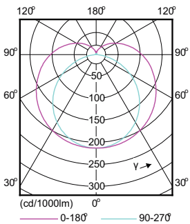
Light Distribution Diagram - 10T8/48-4000 IF 10/1 TAA/NAFTA
