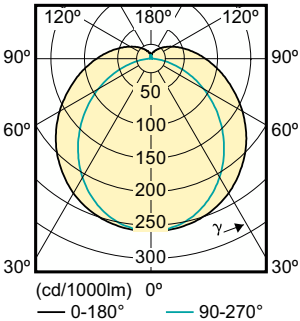
Light Distribution Diagram - MAS LEDtube HF 1500mm HO 25W840 T8
