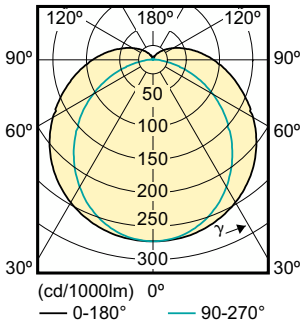
Light Distribution Diagram - MAS LEDtube VLE 600mm 10W840 T8C ROT
