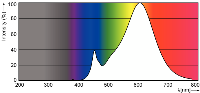
Spectral Power Distribution Colour - LED 6.5W 310mm S19 WW ND 1CT/4
