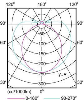
Light Distribution Diagram - LED 6.5W 310mm S19 WW ND 1CT/4
