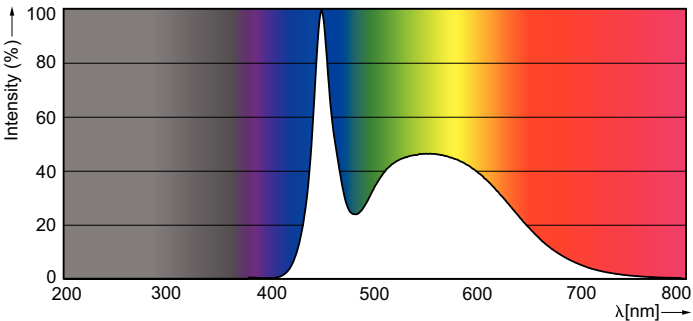
Spectral Power Distribution Colour - MAS LEDtube STD 1200mm 20W865 T8 I
