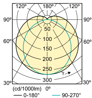
Light Distribution Diagram - MAS LEDtube STD 600mm 10W840 T8 I
