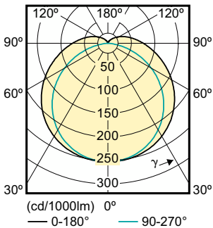
Light Distribution Diagram - CorePro LEDtube 1500mm 20W 865 C
