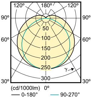
Light Distribution Diagram - CorePro LEDtube 1500mm 20W 865 C
