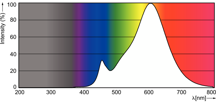
Spectral Power Distribution Colour - MAS LEDspotMV VLE D 3.5-35W GU10 827 25D
