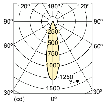
Light Distribution Diagram - MAS LEDspotMV VLE D 3.5-35W GU10 830 25D
