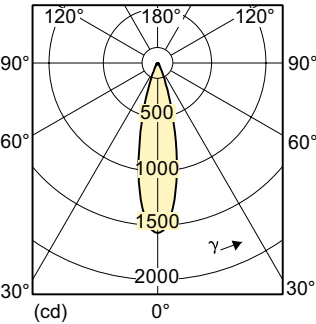
Light Distribution Diagram - MAS LEDspotMV VLE D 4.3-50W GU10 827 25D
