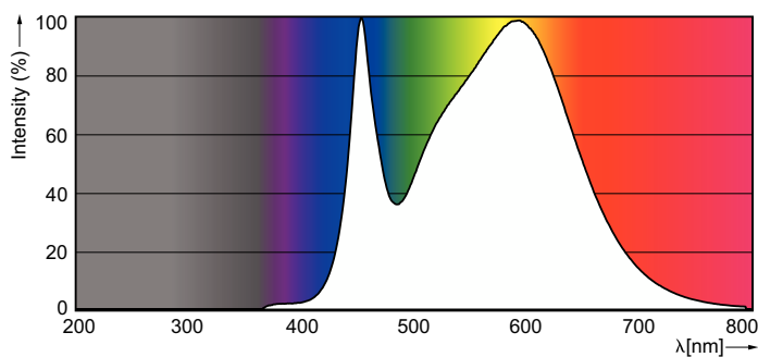
Spectral Power Distribution Colour - MAS LEDspotMV VLE D 4.3-50W GU10 840 25D
