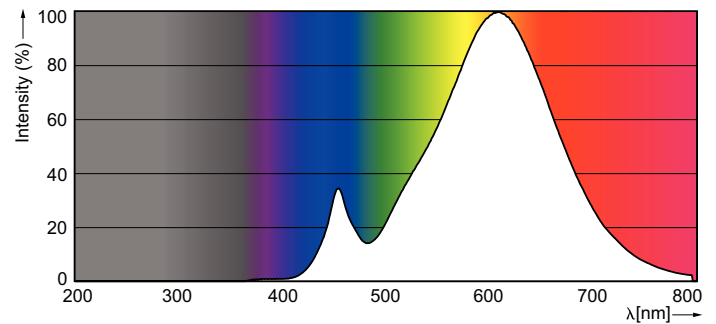
Spectral Power Distribution Colour - MAS LEDspotMV DimTone 4.5-50W GU10 40D
