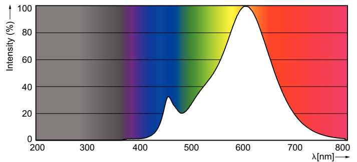
Spectral Power Distribution Colour - MAS LEDspotMV VLE D 3.5-35W GU10 827 40D
