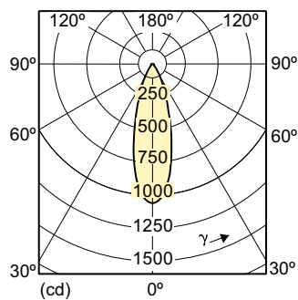
Light Distribution Diagram - MAS LEDspotMV D 5.4-50W GU10 940 40D
