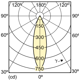
Light Distribution Diagram - MASTER LED 4-35W 2700K MR16 36D CN
