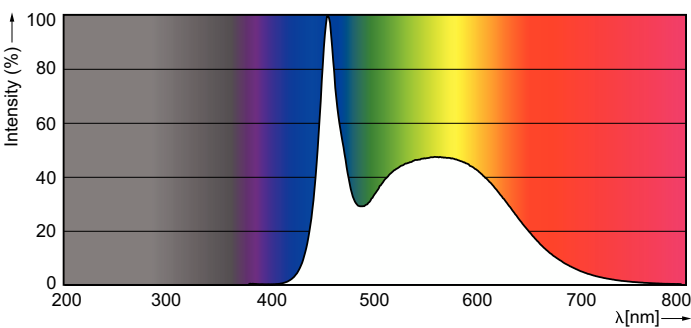
Spectral Power Distribution Colour - MAS LEDtube 1200mm UO 18W 865 T8 RS
