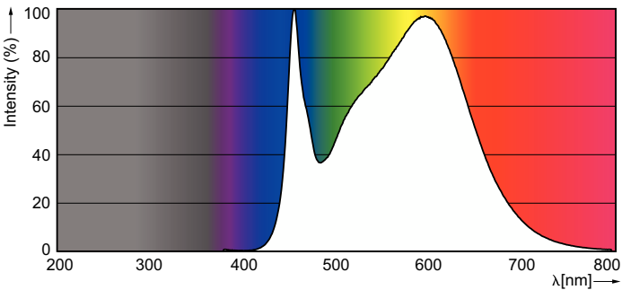
Spectral Power Distribution Colour - MAS LEDtube 1500mm UO 25W 840 T8
