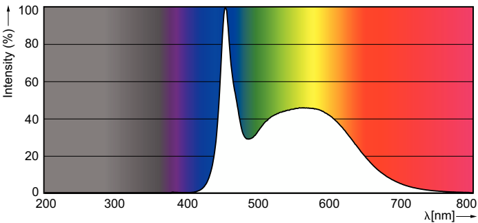
Spectral Power Distribution Colour - MAS LEDtube 1500mm UO 25W 865 T8
