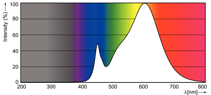
Spectral Power Distribution Colour - MAS LEDtube 600mm 9W 830 T8 RS
