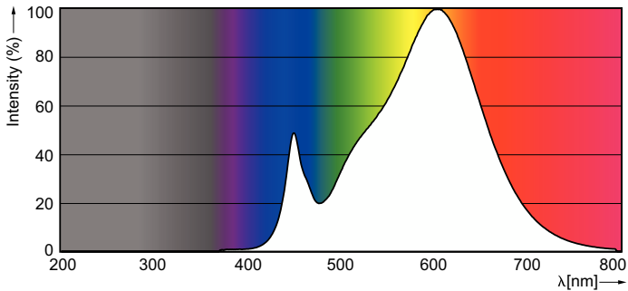
Spectral Power Distribution Colour - MAS LEDtube 600mm 9W 830 T8 RS
