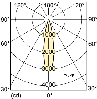
Light Distribution Diagram - MASTER LED 8.0-50W+ 827 MR16 24D Dim CN
